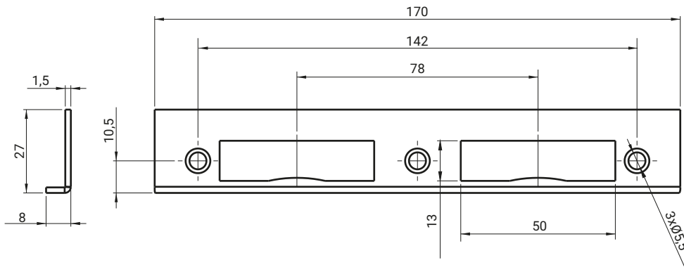
Latching element
