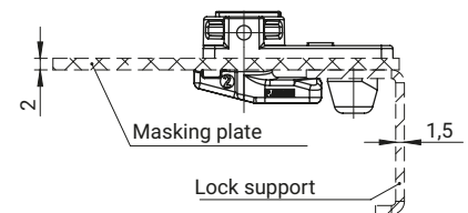
Auxiliary installation plan
