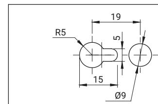
Mounting holes
