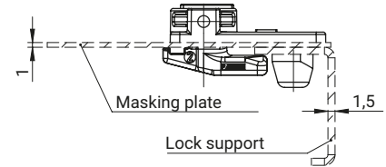
Auxiliary installation plan
