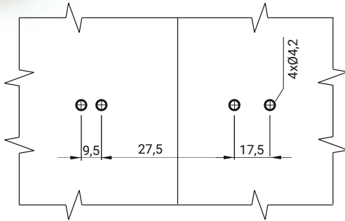
Mounting hole
