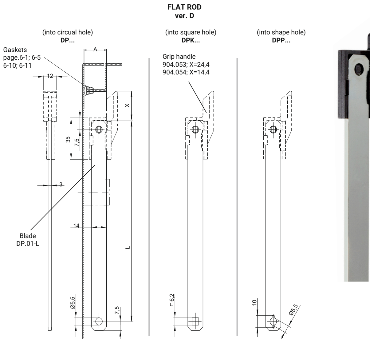
GRIP HANDLE 1C.904.053
