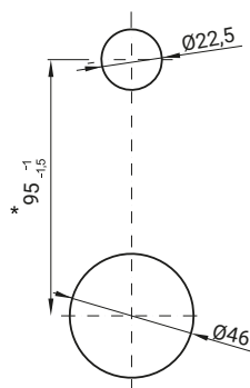
Mounting hole
