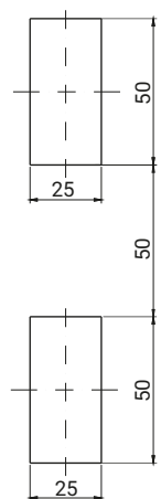
Mounting hole
