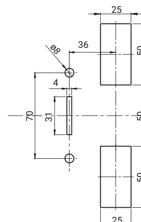
Mounting hole
