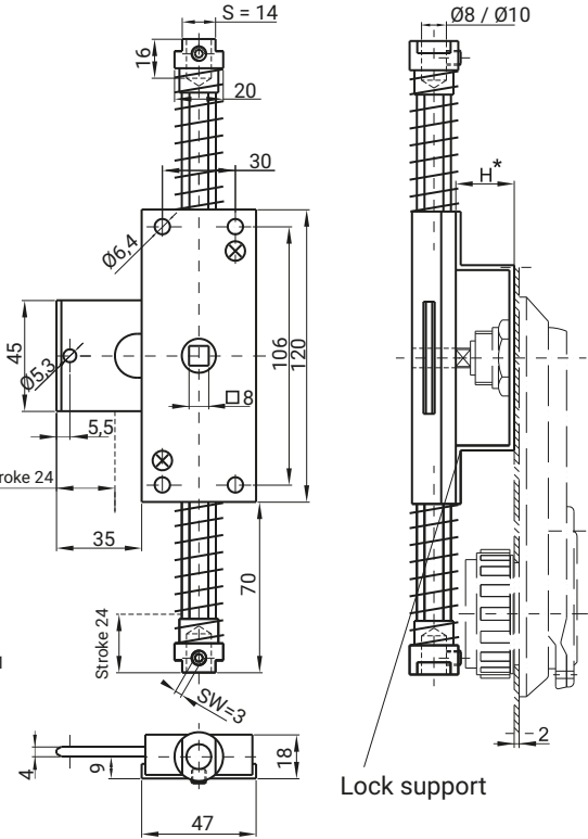
ZW8 (with hole ø8) ZW10 (with hole ø10)
