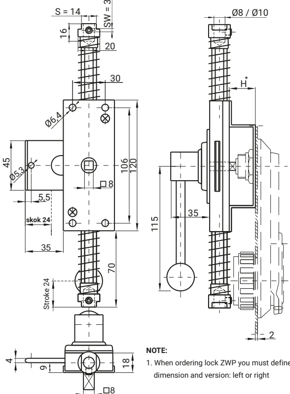
ZWP8 (with hole ø8) ZWP10 (with hole ø10)
